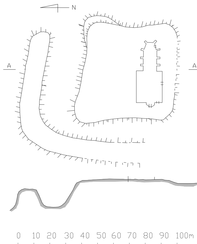
Sl. 12 Donja Glogovnica, tlocrt i presjek gradišta (crtež: T. Tkalčec) Fig. 12 Donja Glogovnica, layout and cross-section of the fortification (drawing: T. Tkalčec)
