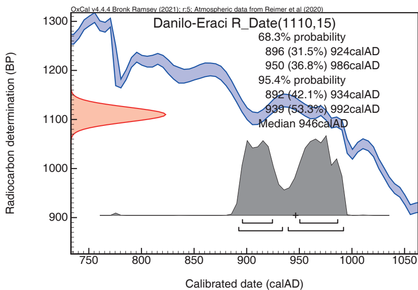
Sl. 6 Kalibrirani 14 C datum ulomka ljudske lubanje (OxCal v4.4.4 Bronck Ramsey 2021; r:5; Atmospheric data from Reimer et al. 2020) (izradila: K. Botić) Fig. 6 Calibrated 14 C date of a human skull fragment (OxCal v4.4.4 Bronck Ramsey 2021; r:5; Atmospheric data from Reimer et al. 2020) (made by: K. Botić)
